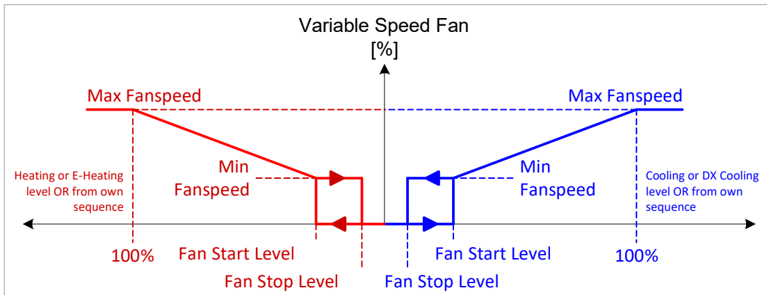
Fig. 22. Variable-speed fan speed depending on control demand
