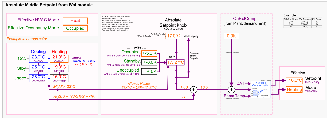
Fig. 25. Absolute Setpoint Adjustment
