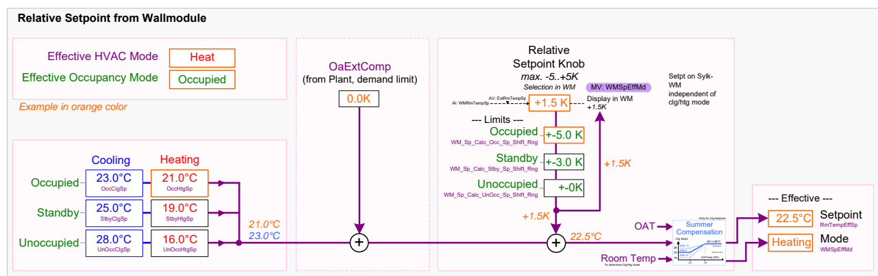
Fig. 24. Relative Setpoint Adjustment
