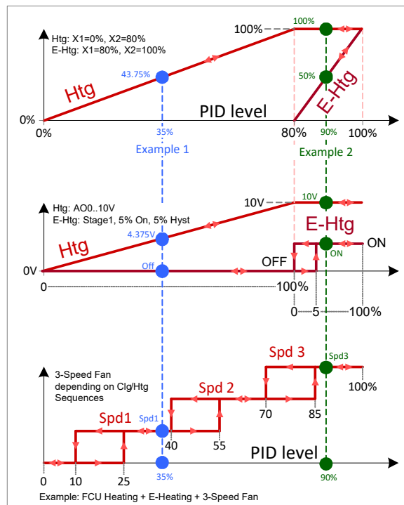
Fig. 21. Multi-speed fan, Heating and E-Heating control Example
