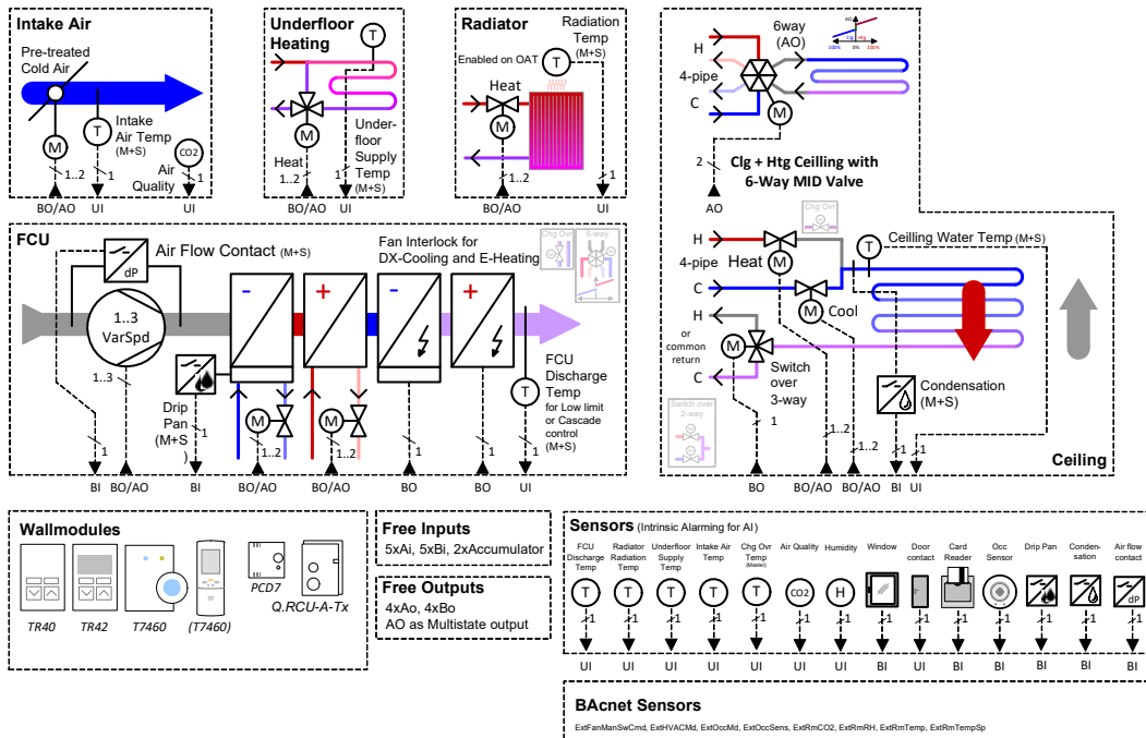
Fig. 2. Application Overview
