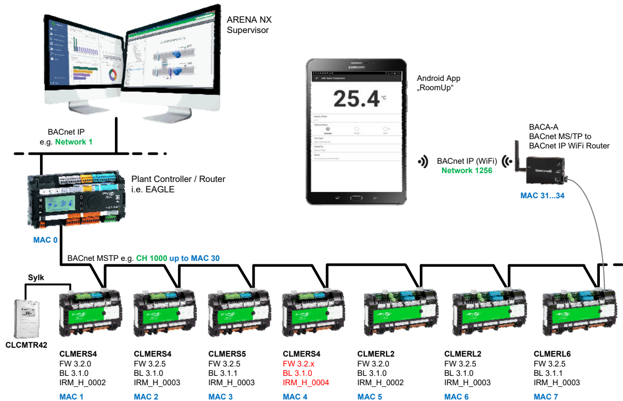
Fig. 1. System Architecture
