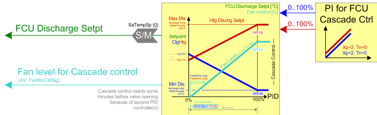
Fig. 17. Example 1: Temperature Configuration via Cascade Control
