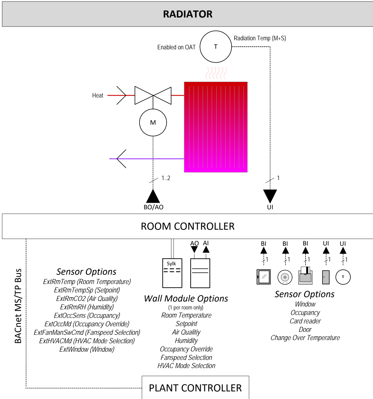
Fig. 8. Radiator control application
