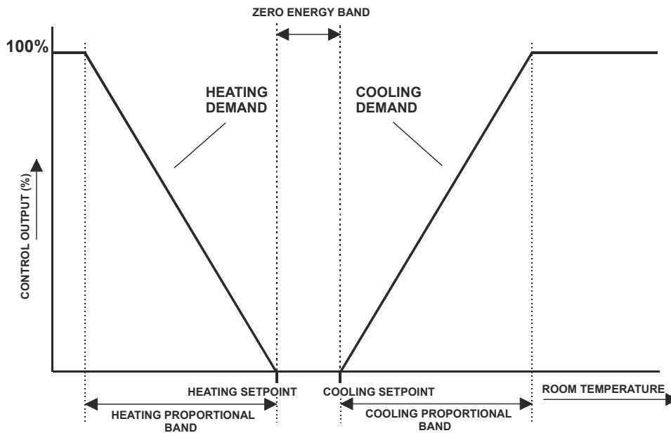
Fig. 15. Control sequence diagram (P-Control Example)
