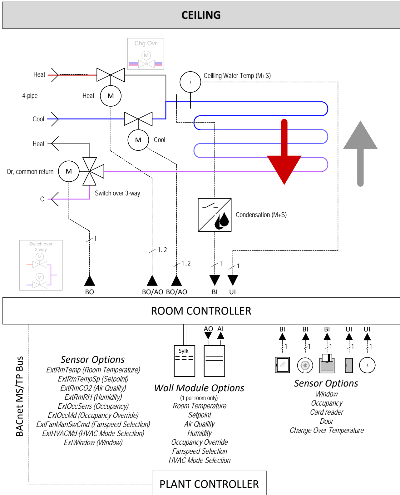
Fig. 4. Ceiling control application
