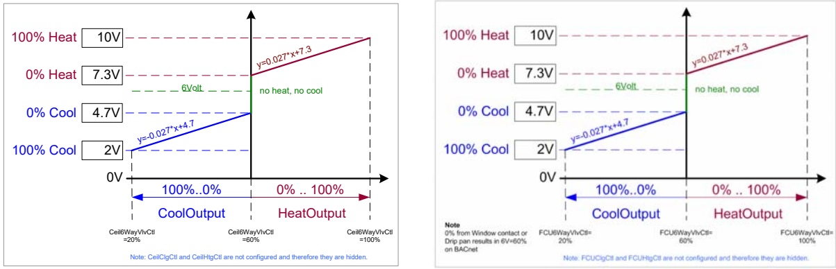
Fig. 36. 6-Way Valve output for Cooling and Heating
