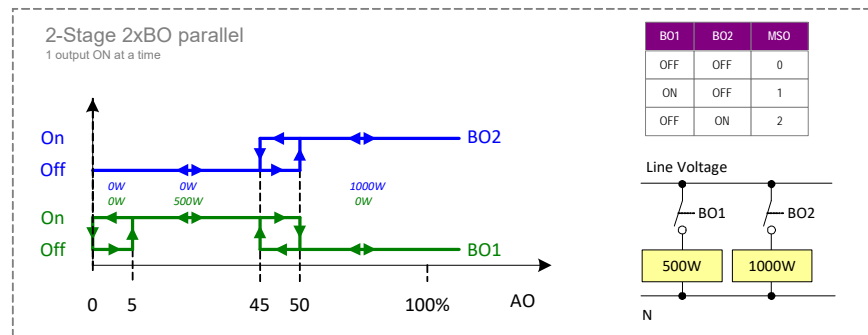
Fig. 27. Free Output: 2-Stage 2xBO parallel
