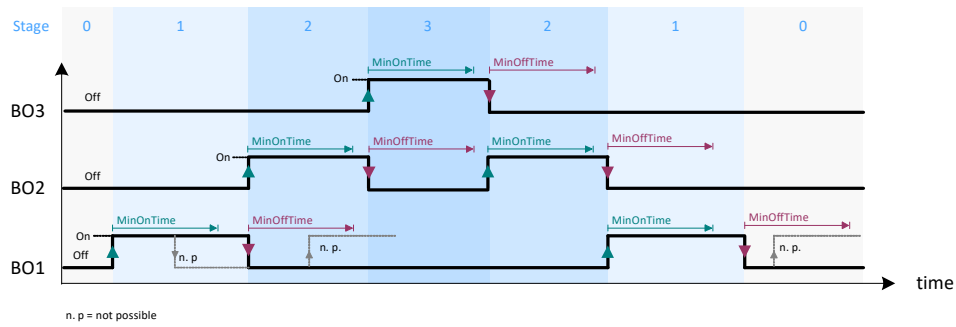
Fig. 32. 3-Stage Output: Min On/Off Time Switching Behavior
