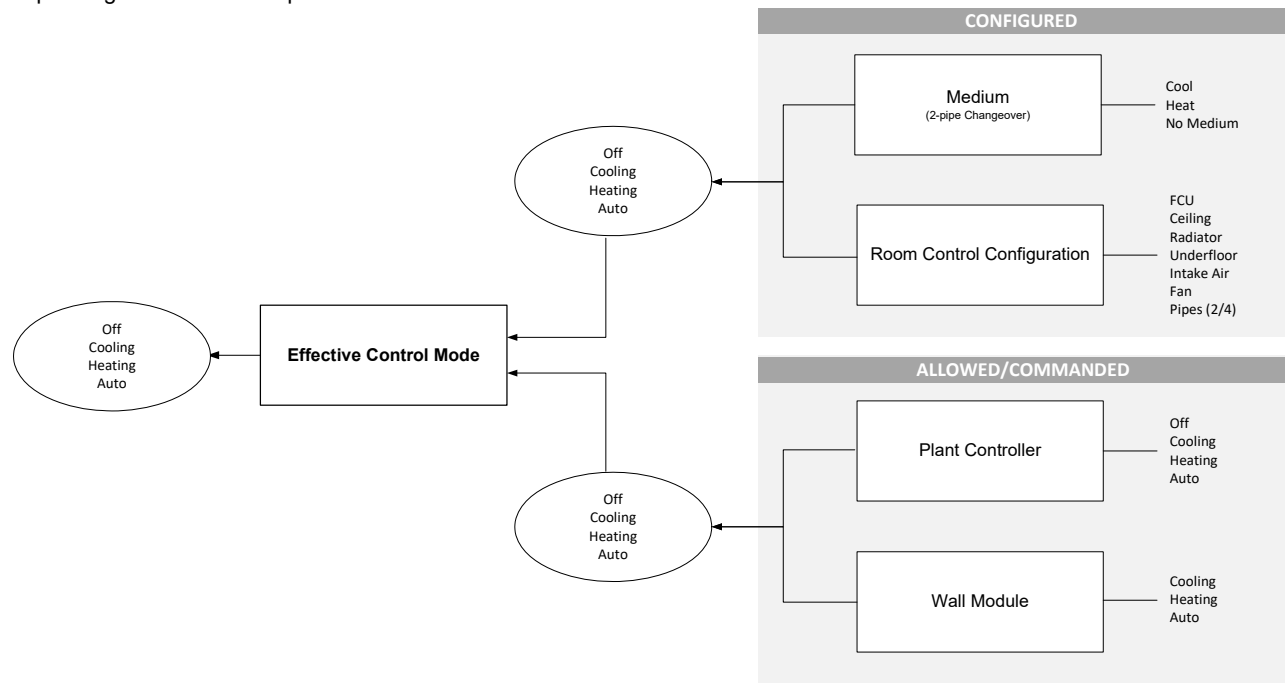
Fig. 13. Effective Control Mode
