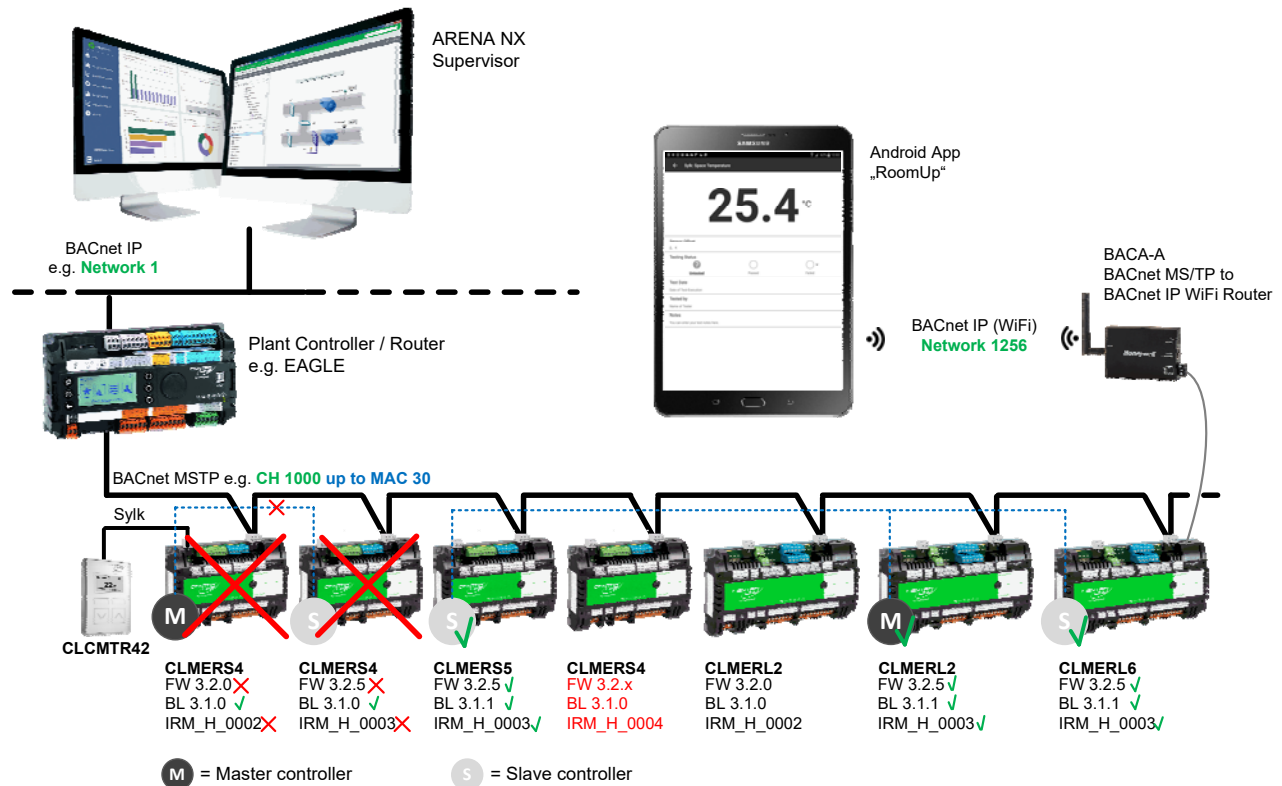
Fig. 37. Master-Slave System Architecture
