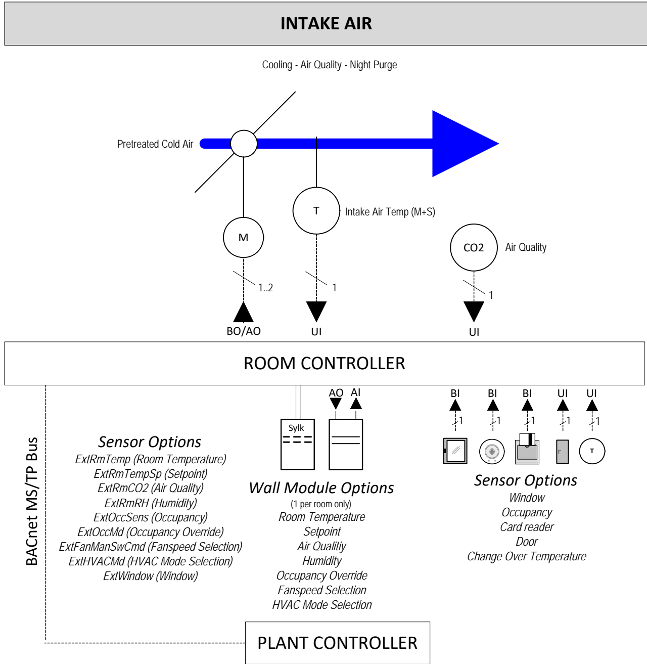
Fig. 10. Intake Air control application
