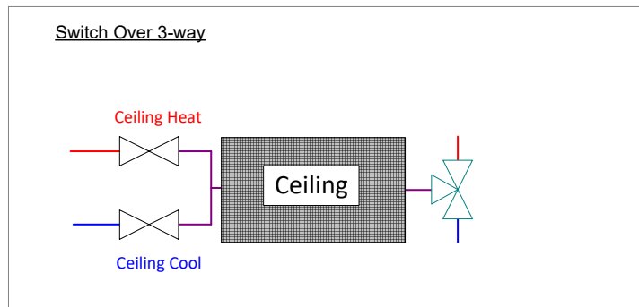
Fig. 7. Ceiling Switch-Over Configuration with 3-way valve
