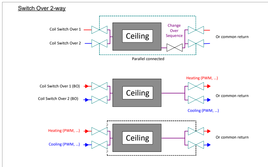
Fig. 6. Ceiling Switch-Over Configuration with 2-way valve
