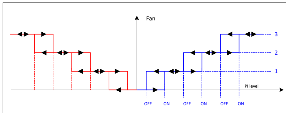
Fig. 20. Multi-speed fan switching depending on control demand
