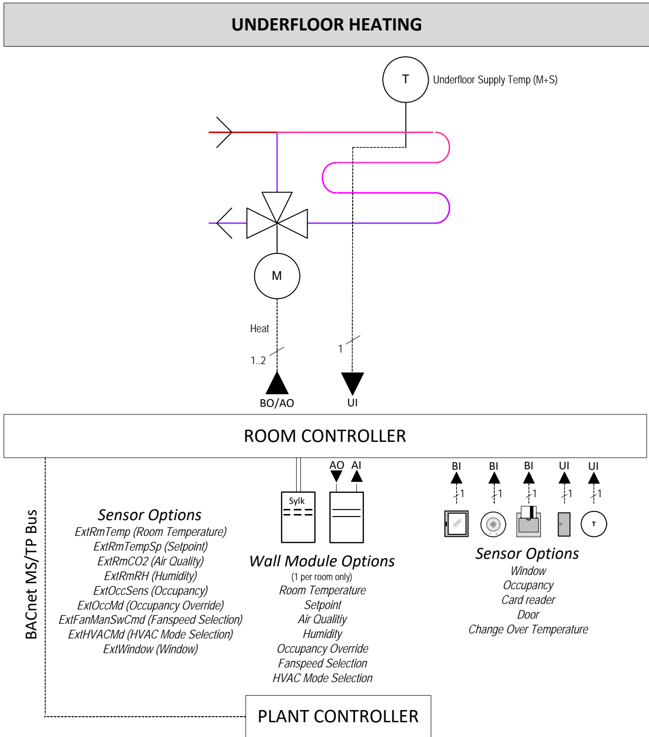
Fig. 9. Underfloor Heating Control Application
