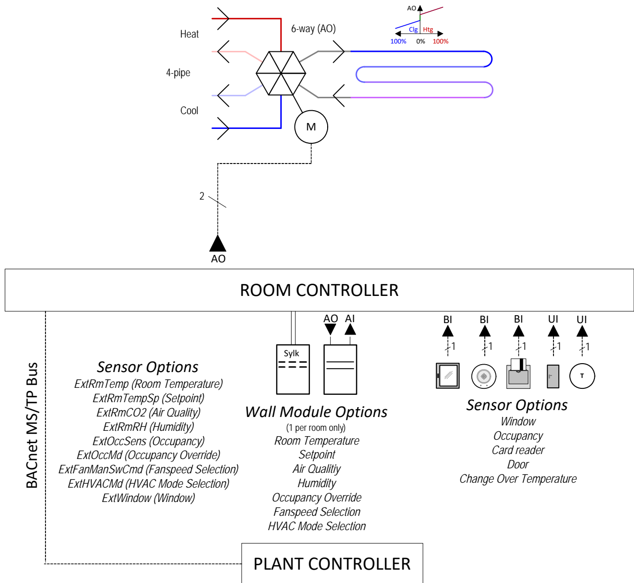
Fig. 5. Ceiling 6-Way-MID Valve control application
