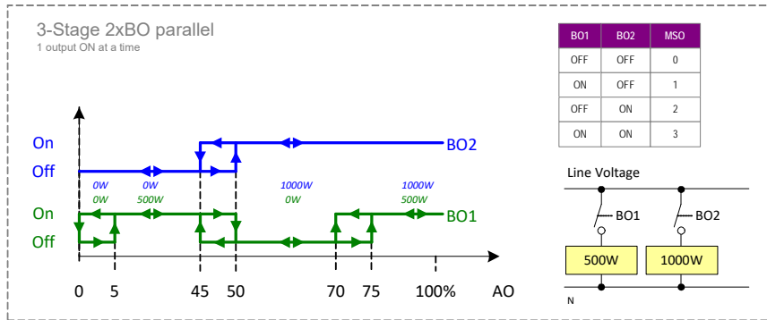
Fig. 29. Free Output: 3-Stage 2xBO parallel
