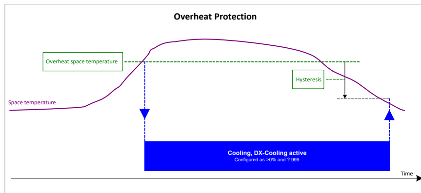
Fig. 12. Overheat Protection Example
