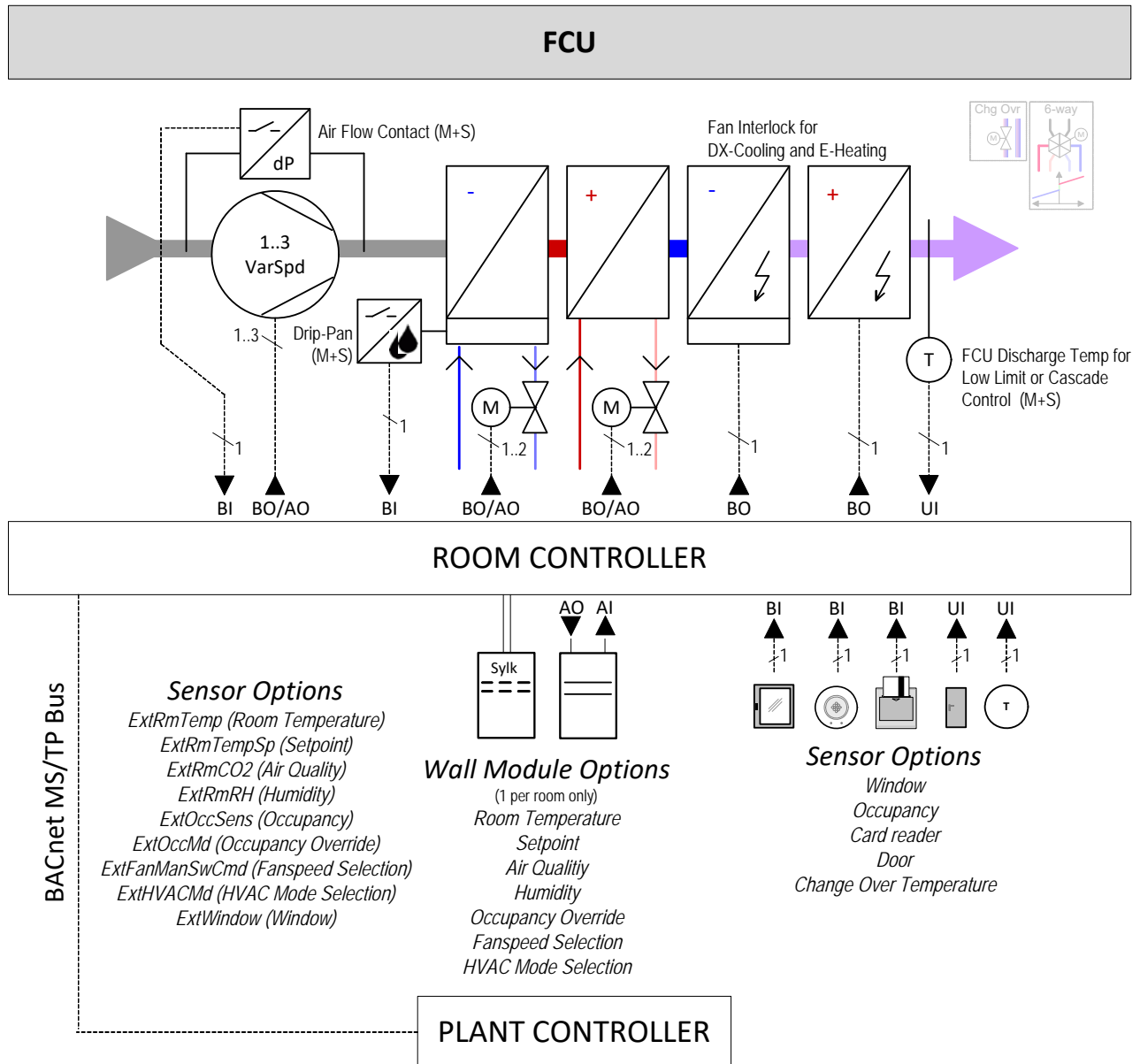
Fig. 3. Fan Coil Unit control application
