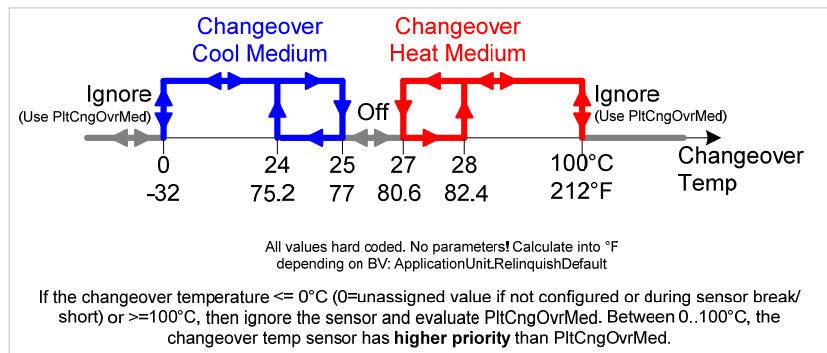
Fig. 34. Cooling / Heating Changeover Temperature Sensor Behavior
