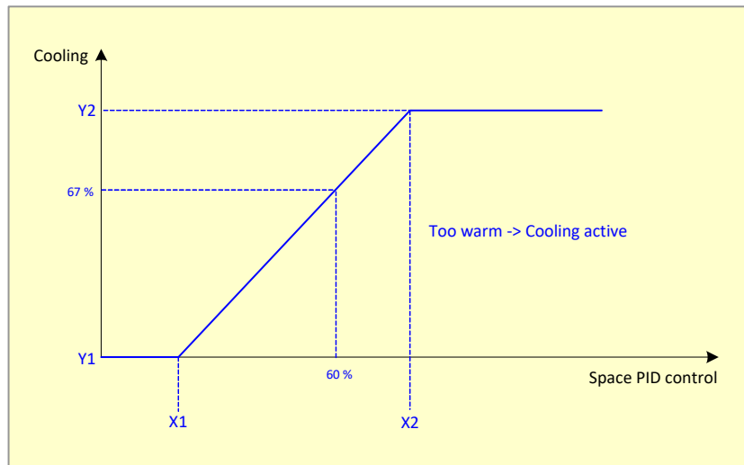
Fig. 16. Sequence Configuration (FCU Cooling Example)
