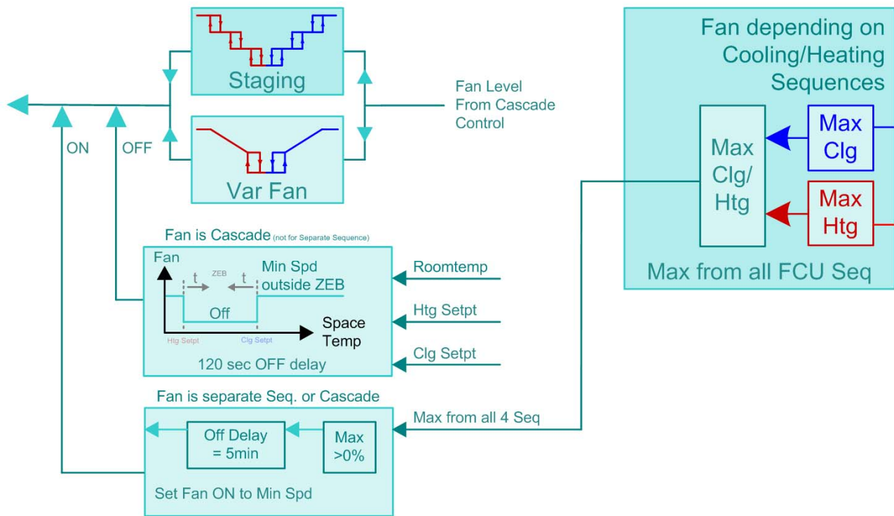
Fig. 18. Example 2 Temperature Configuration via Cascade Control
