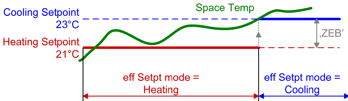
Fig. 14. Effective Setpoint Mode
