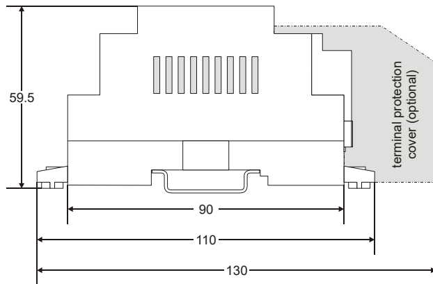
Fig. 2. Excel 10 W7754 dimensions (in mm)
