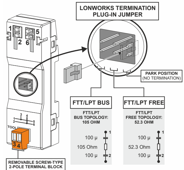
Fig. 9. LonWorks connection and termination module
