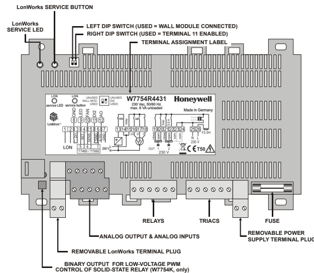
Fig. 1. Excel 10 W7754 FCU Controller (w/o opt. cover)
