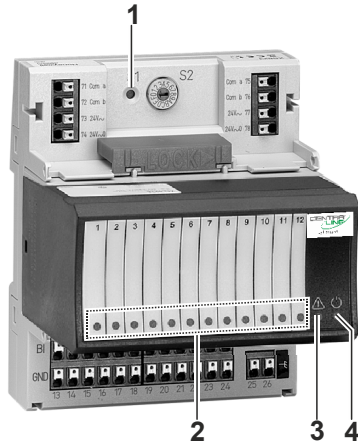
Fig. 15. CLIO823A LONWORKS Bus BI Module (shown with XS823 terminal socket)
