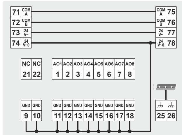
Fig. 11. CentralLine LONWORKS Bus Analog Output Modules (schematic)
