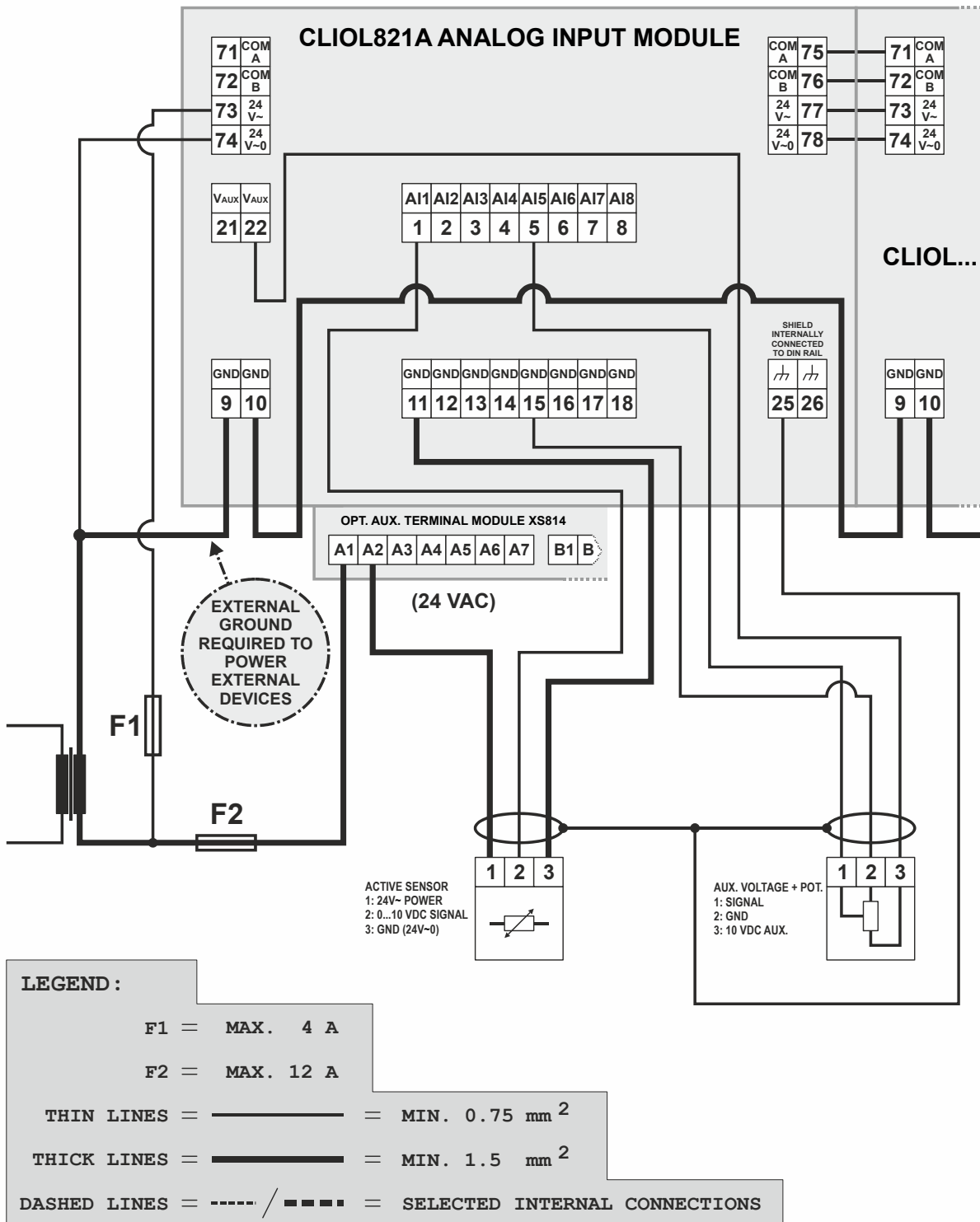
Fig. 8. CLIO821A LonWorks Bus AI Module, wiring example 1: Active sensor and potentiometer
