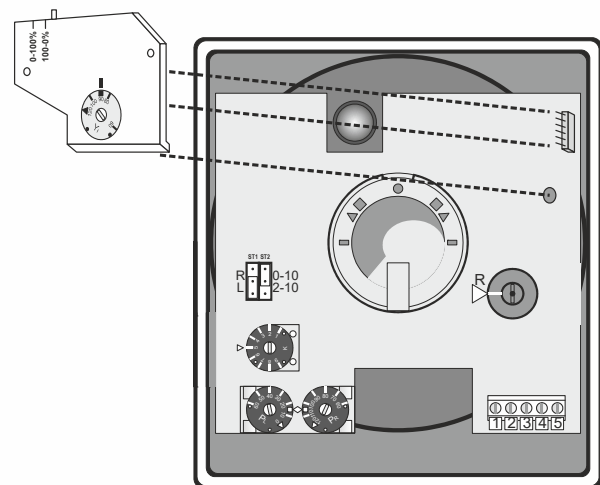
Fig. 6. Mounting VMU1
