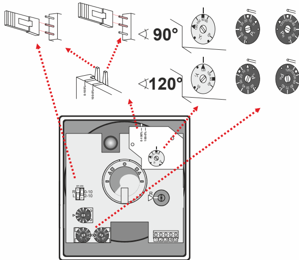
Fig. 7. Adjusting settings
