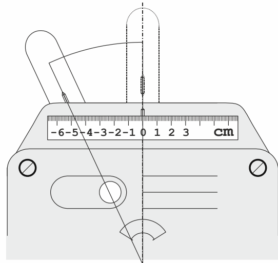
Fig. 5. Verifying setting at lever
