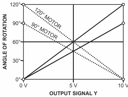
Fig. 8. Output signal Y and angle of rotation with VMU1
