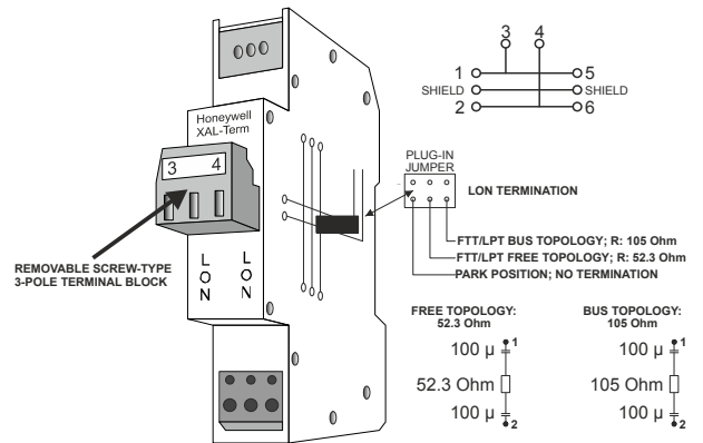
Fig. 17. XAL-Term Connection and Termination Module.
