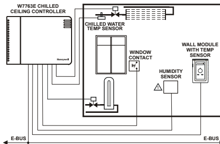
Fig. 2. Typical application
