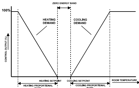
Fig. 1. Operational sequence
